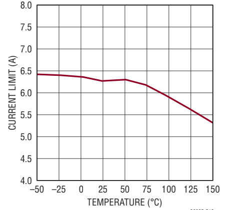
Bottom FET Positive Current Limit vs Temperature
