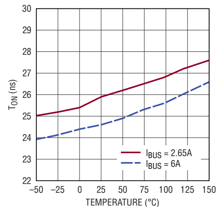
Top FET Minimum On-Time
